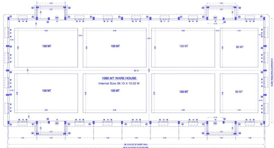
1080 MT WARE HOUSE UNIT PLAN
