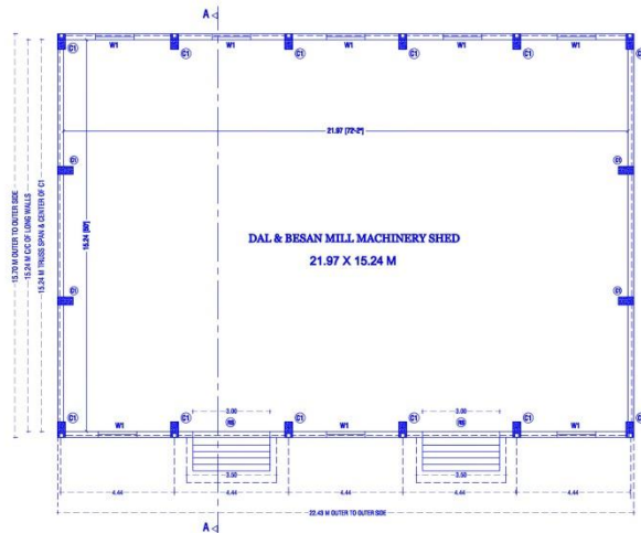
DAL & BESAN MILL MACHINERY SHED PLAN
